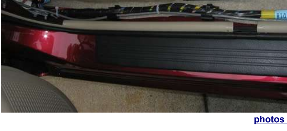
20) OBD2 cable running along door sill to driver's seat 21) cautionary note: the version 3 has two 10 pin sockets, one grey for the programmer and 1 black for the MFD or NAV. The grey programmer plug cannot possibly squeeze into the black MFD socket, but the black MFD/NAV plug will fit loosely in the grey programmer socket. Do NOT do this! Damage is likely. Both MFD and OBD2 plugs are black and go into the 2 black sockets next to each other.
