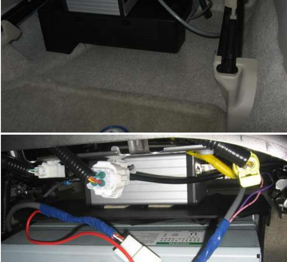
8) Installed CAN-View box on top of NAV box. View from the center of the rear seat
