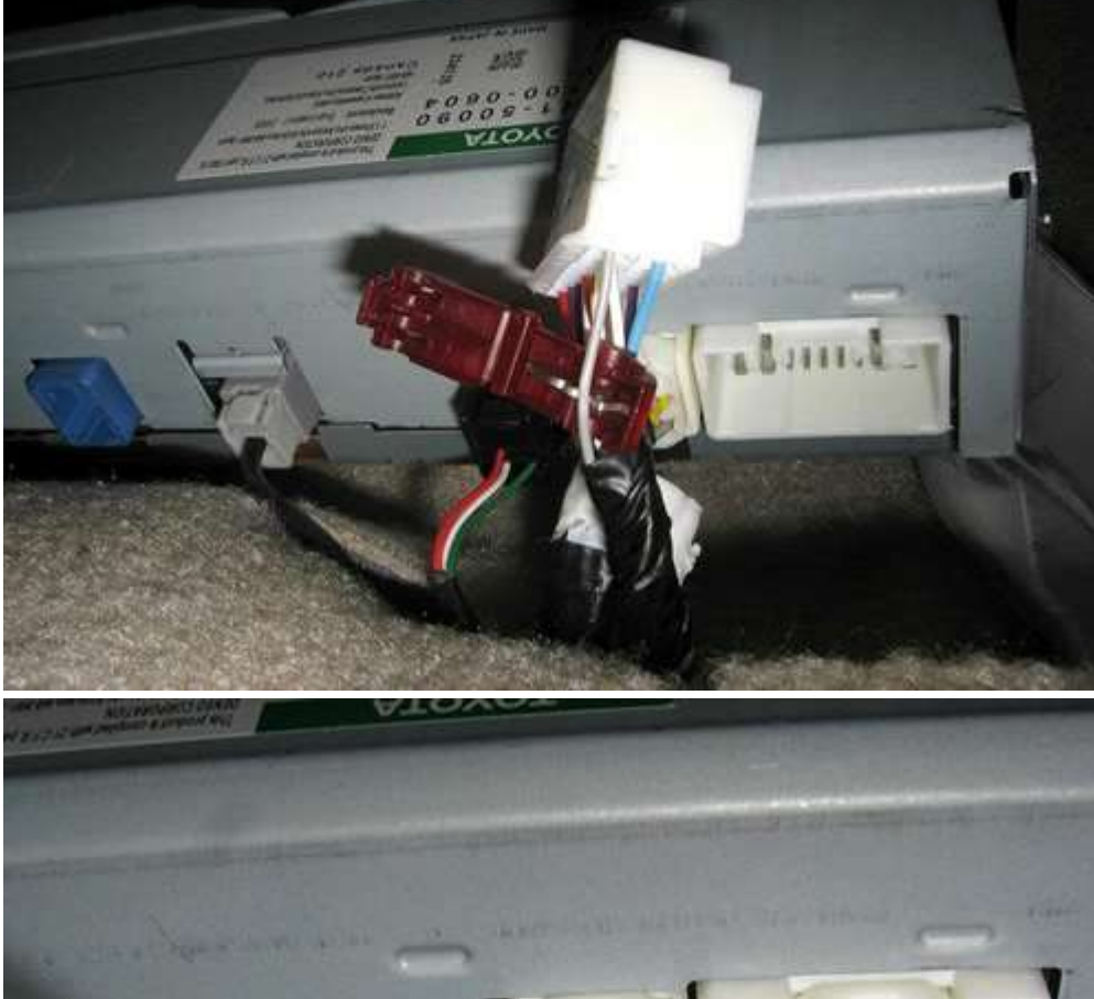
2) The N2 plug removed from NAV to install tap on grey wire. Plug was removed from the NAV unit and turned upside down to get easier access to the grey wire. If you choose to remove N2, you will lose your NAV region settings and will have to re-enter them later. Make sure the T-tap is firmly crimped with a large pair of pliers
