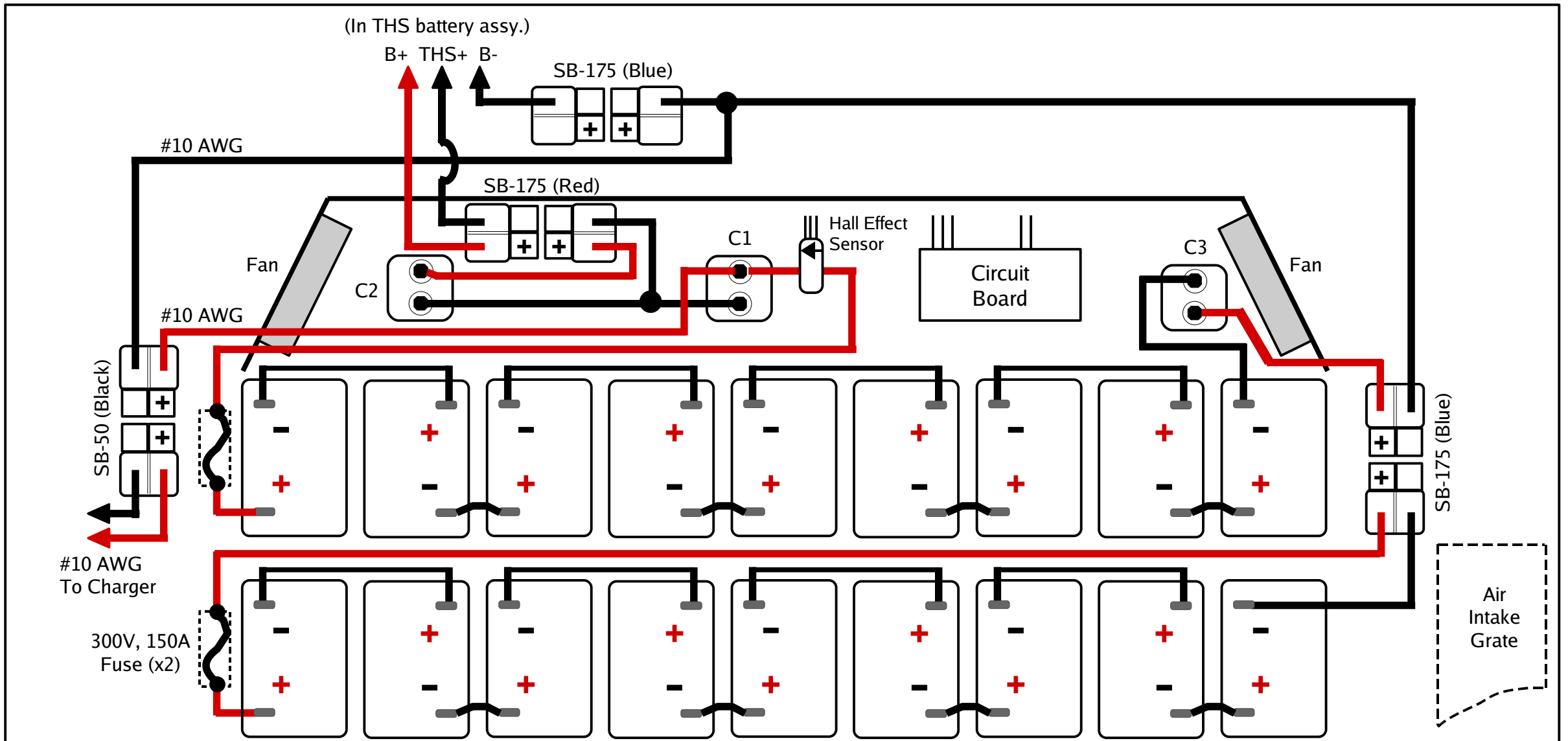
(18) BB Battery Corp. EVP20-12 12Volt, 20Ah Lead-Acid Batteries
